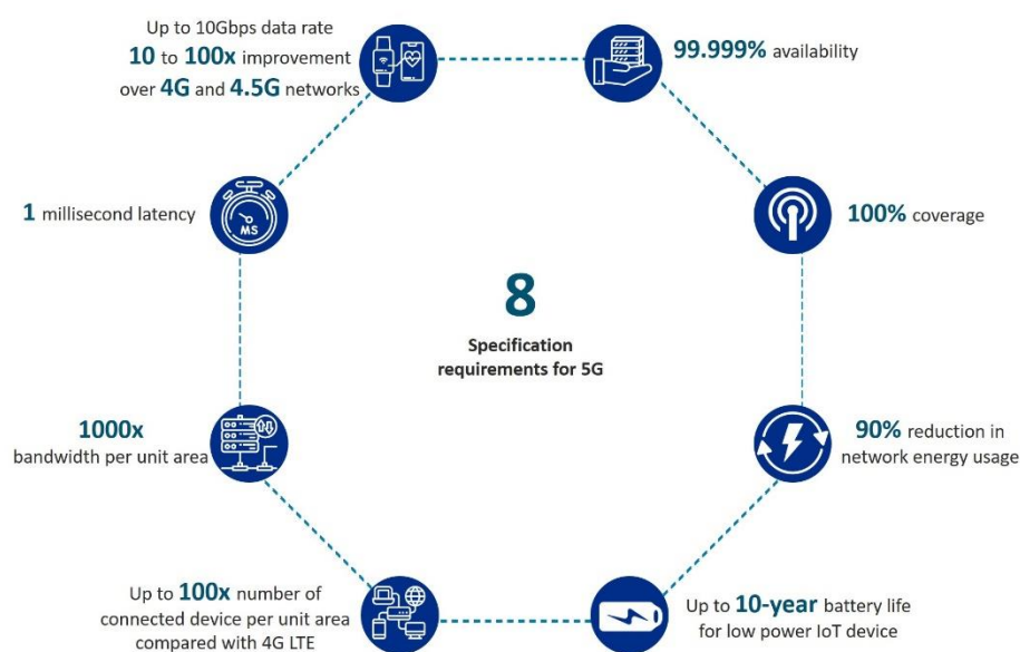
Figure 1: 5G Requirements
