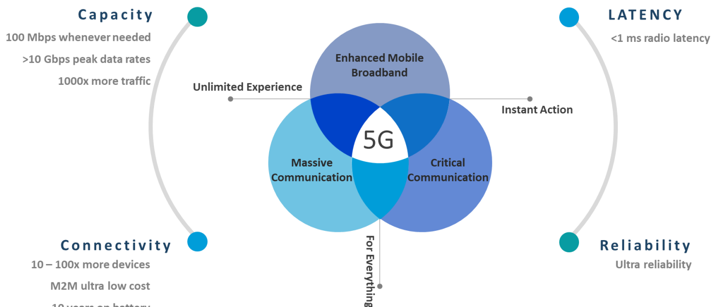
Figure 6: 5G Features
